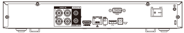
DHI-HCVR7104H-4K
